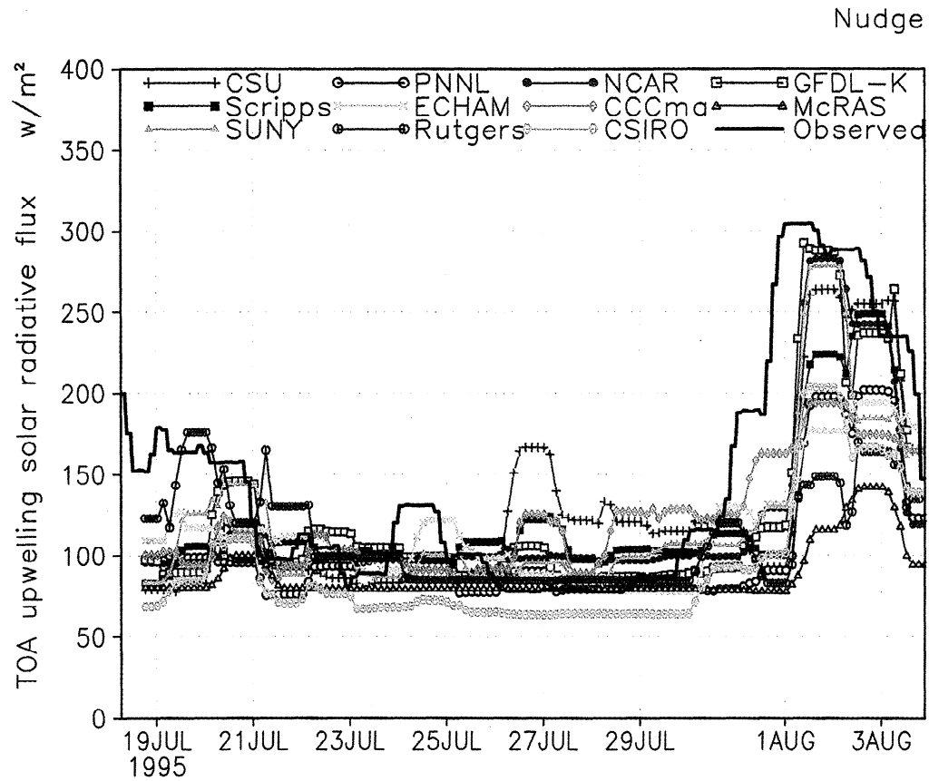
Plate 15. Upward 24 hour running mean solar radiative flux at the top of the atmosphere ( W m^{-2} ) as observed and as simulated by each model driven by the forcing shown in Plates 1 and 2 with nudging toward the analyzed temperature and humidity.
