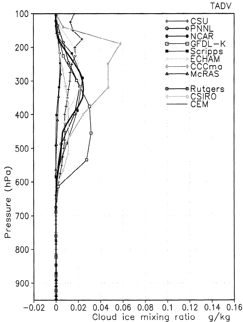
Plate 14. Vertical profile of the 17 day mean cloud ice mixing ratio (g/kg) simulated by each model using the baseline forcing shown in Plates 1 and 2.
