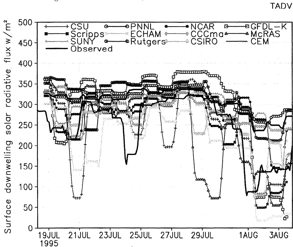
Plate 8. Downward 24 hour running mean solar radiative flux at the surface ( \text{W m}^{-2} ) as simulated by each model using the baseline forcing shown in Plates 1 and 2, and as observed.
