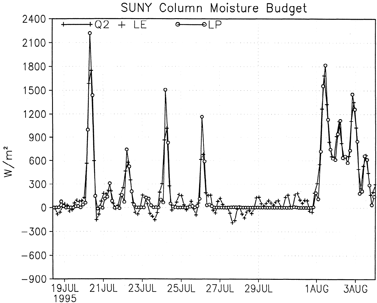
Figure 3. Column moisture budget (in W m^{-2} of latent heat) according to the (a) SUNY and (b) LLNL objective analyses. Q2 is the latent heat of evaporation multiplied by the column integral of the apparent moisture sink. LP and LE are the latent heat of evaporation multiplied by the precipitation rate and evaporation rate, respectively.
