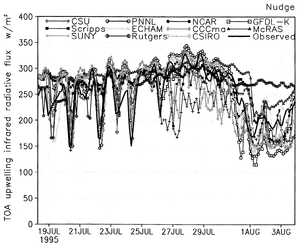
Plate 16. Outgoing longwave radiative flux at the top of the atmosphere ( W m^{-2} ) as observed and as simulated by each model driven by the forcing shown in Plates 1 and 2 with nudging toward the analyzed temperature and humidity.
