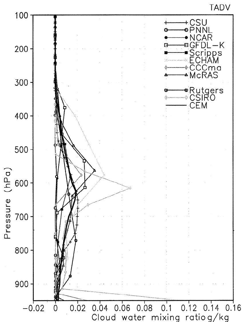
Plate 13. Vertical profile of the 17 day mean cloud water mixing ratio (g/kg) simulated by each model using the baseline forcing shown in Plates 1 and 2.
